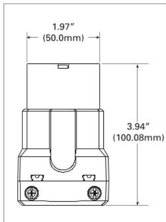
Figure 2. AHCL1430C
