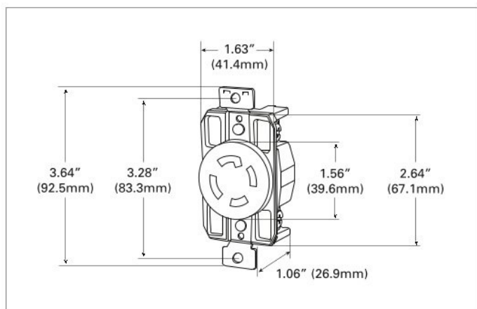
Figure 4. AHCL1430R
