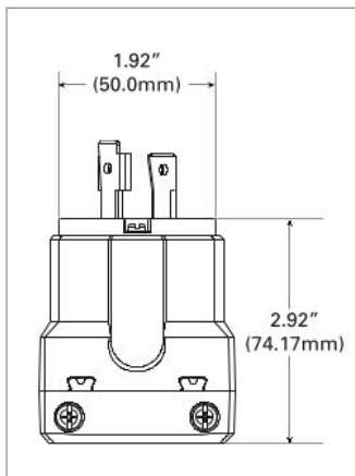
Figure 1. AHCL1430P
