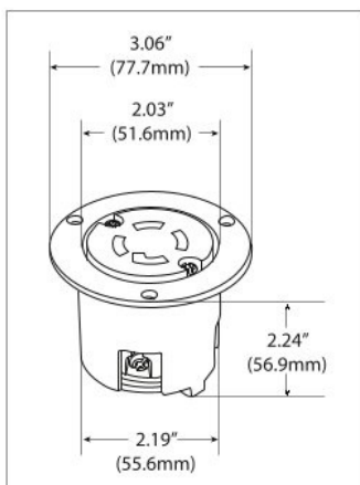
Figure 5. AHCL1430FO
